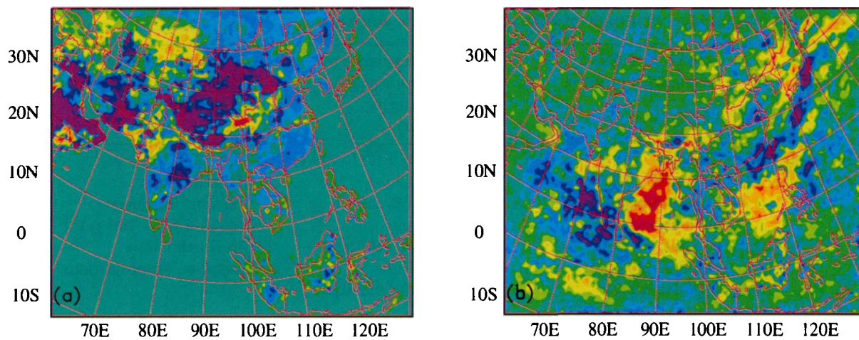
Fig. 8. Geographical distributions of annual mean temperature (left, units: °C) and precipitation (right, units: mm). (a) and (b) as simulated by the TEACOM regional climate model with black carbon (sensitivity minus control) (from Wu et al., 2004).
