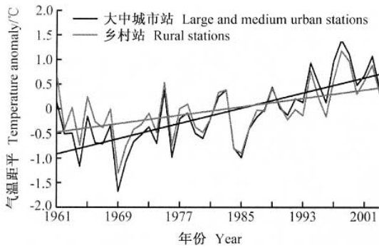
图 2 1961~2003 年期间河北省地区大中城市站、乡村站平均的年平均气温距平 Fig. 2 Annual mean air temperature anomalies for large and medium urban stations (LMS), rural stations (RS) over Hebei Province (1961—2003)
