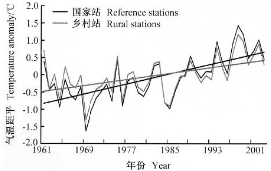
图 4 1961~2003 年期间河北省地区国家站、乡村站平均的年平均气温距平 Fig. 4 Annual mean air temperature anomalies for basic/reference stations (US), rural stations (RS) over Hebei Province (1961—2003)
